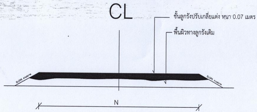
SECTION A
