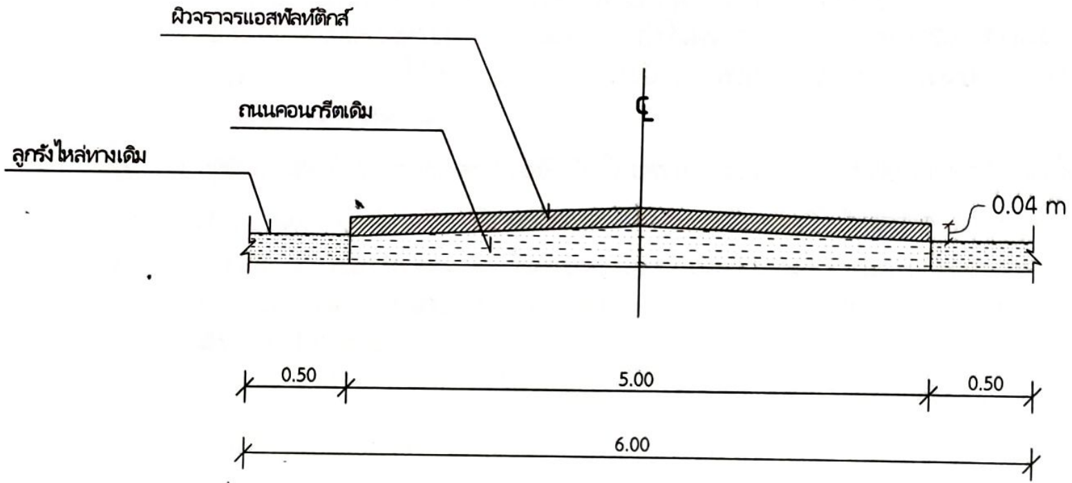
SECTION
